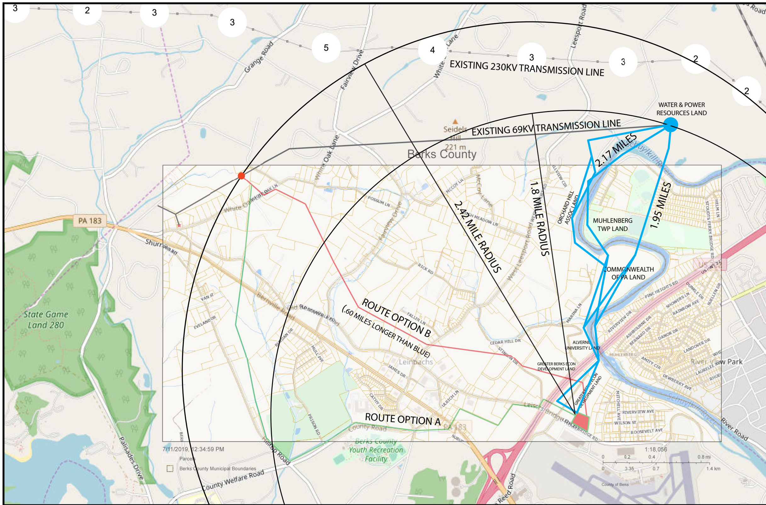
2019 FIRST ENERGY/AFS 69KV TRANSMISSION LINE FOR AIRPORT INDUSTRIAL PARK RADIAL SUBSTATION
